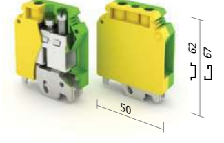
UT1-35PE(T)
