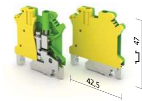
UT1-4PE(T)
