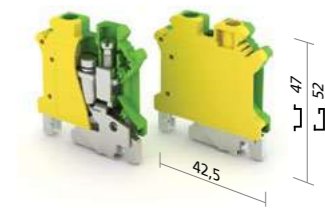
UT1-6PE(T)
