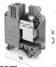
UT1-35(T)
